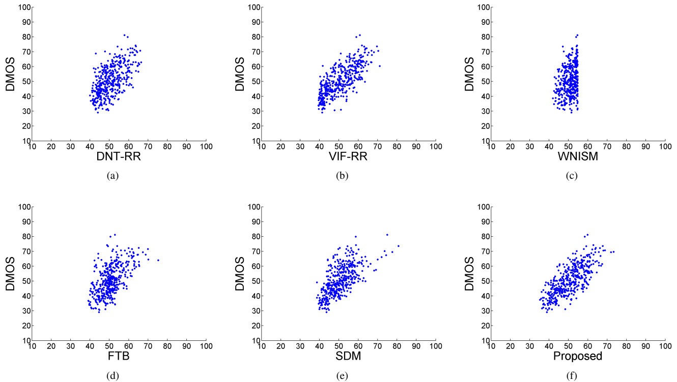
Fig. 8. Scatter plots of the DMOS vs objective RR-IQA scores (after nonlinear regression) for compressed SCIs (including JPEG, JPEG2000 and layer segmentation based coding).
