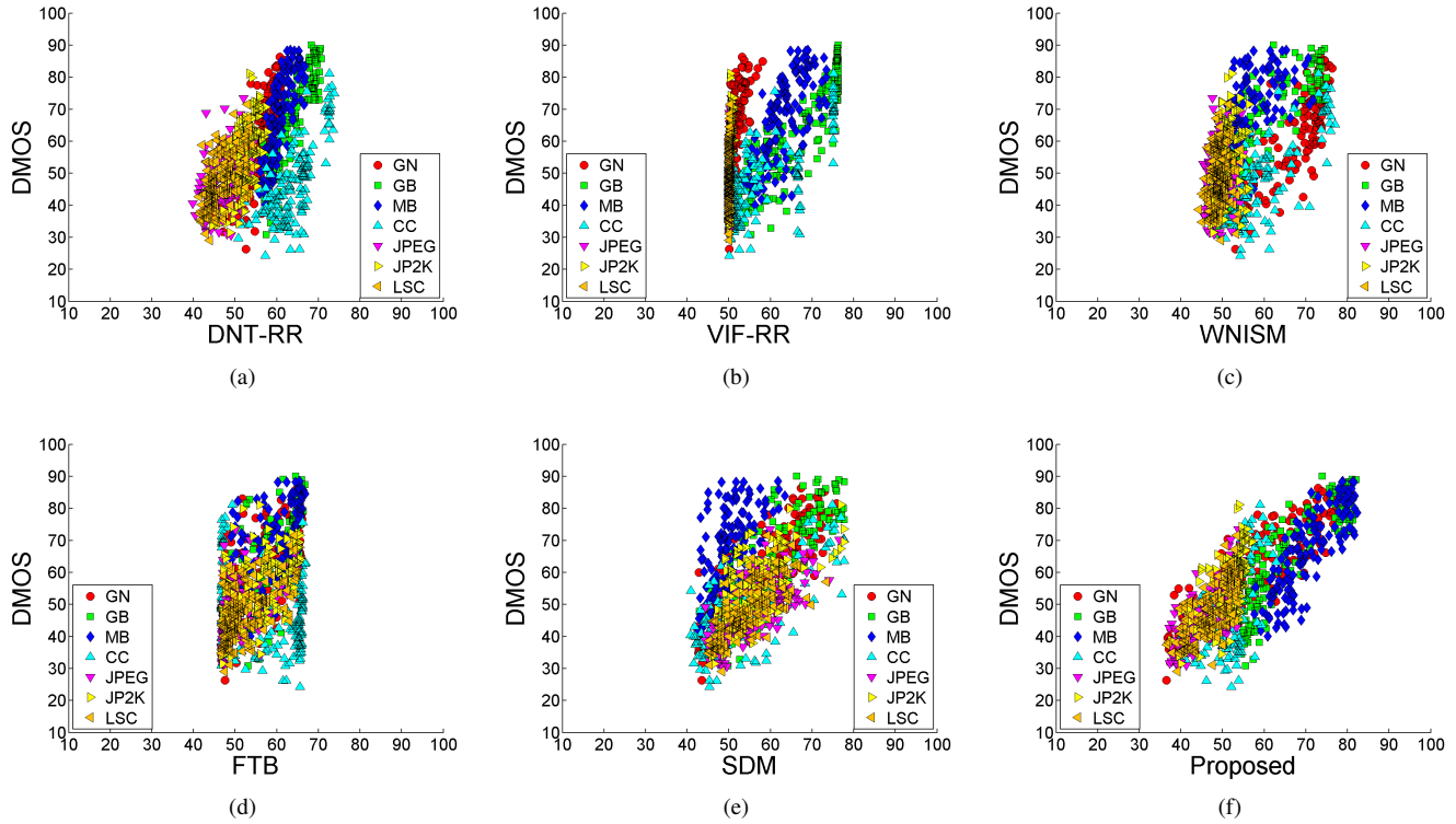
Fig. 7. Scatter plots of the DMOS vs objective RR-IQA scores (after nonlinear regression) for all SCIs.
