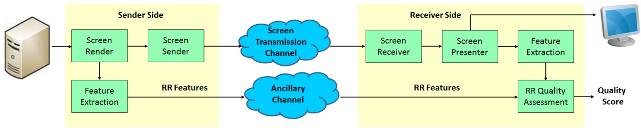
Fig. 2. General framework of an SCI RR-IQA system.
