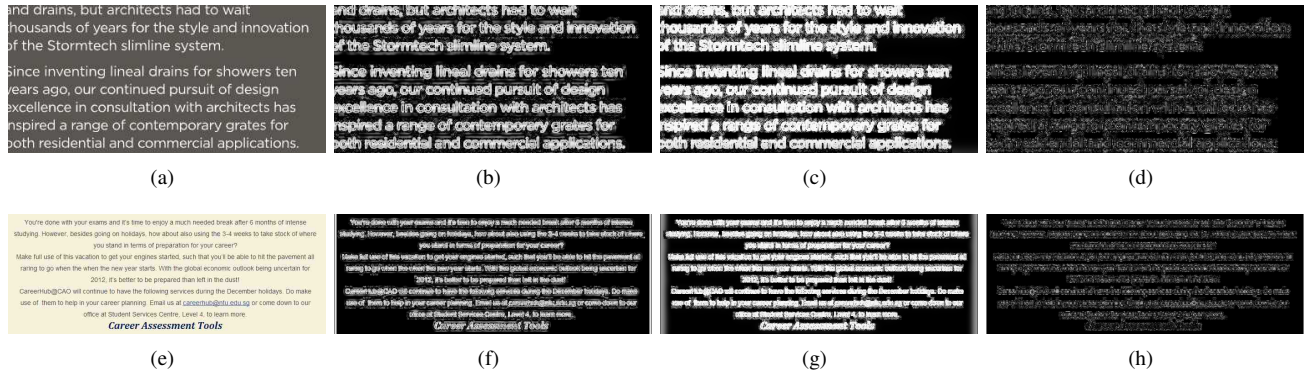
Fig. 5. Illustration of S_G maps generated by comparing the input and the low-pass filtered SCIs with different parameters. (a)(e) Distorted SCIs as the input; (b)(f) \sigma = 5.5 ; (c)(g) \sigma = 11 ; (d)(h) \sigma = 1.0 .
